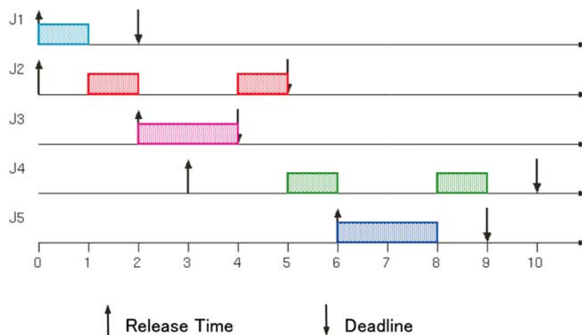
Figure A.1 – EDF scheduling
